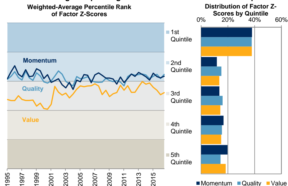
Exhibit 4: Holding Multiple Single-Factor Indices Lowers Factor Exposures
